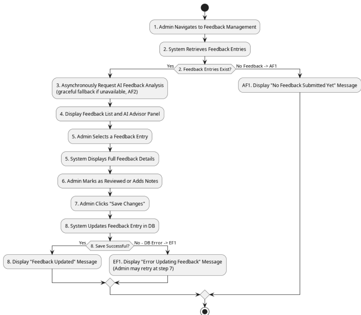
Figure 2.31: Activity Diagram for Manage Feedback
