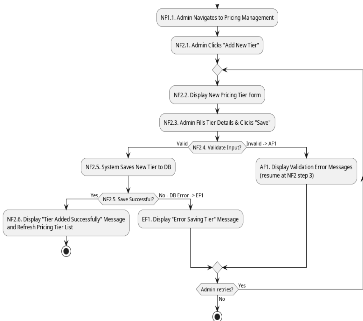
Figure 2.17: Activity Diagram for Manage Pricing Panel (Add New Tier Flow)
