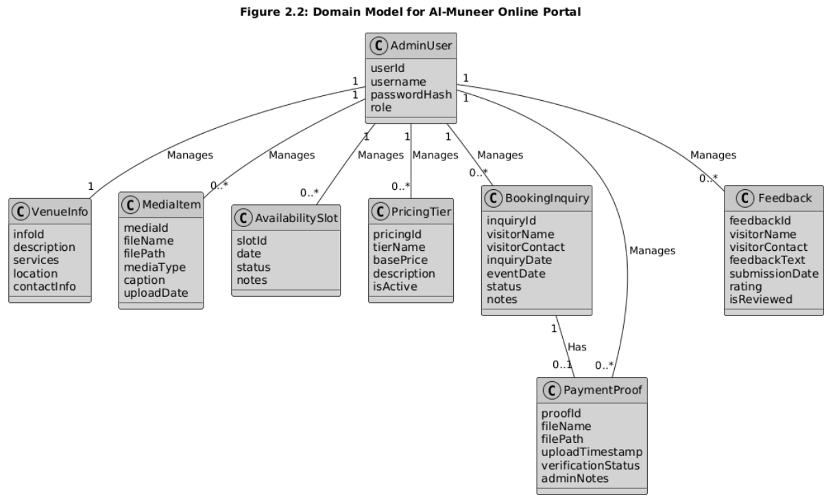
Figure 2.2: Domain Model for AI-Muneer Online Portal
